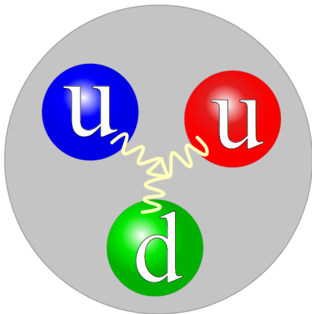
Figure: quark model
