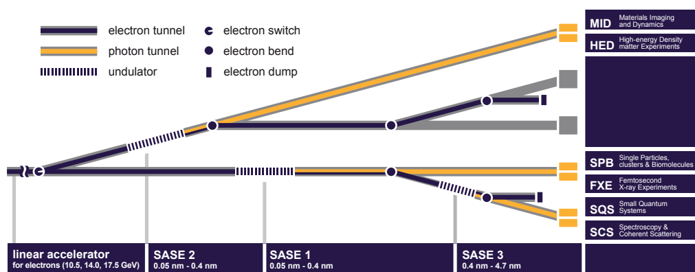
Figure 4.1: Layout of the photon beam systems at the European XFEL facility.
